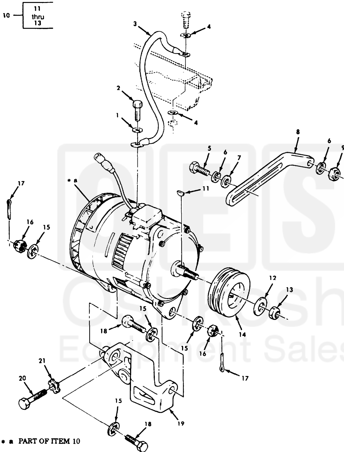
Figure 31. 60-Ampere Alternator.
